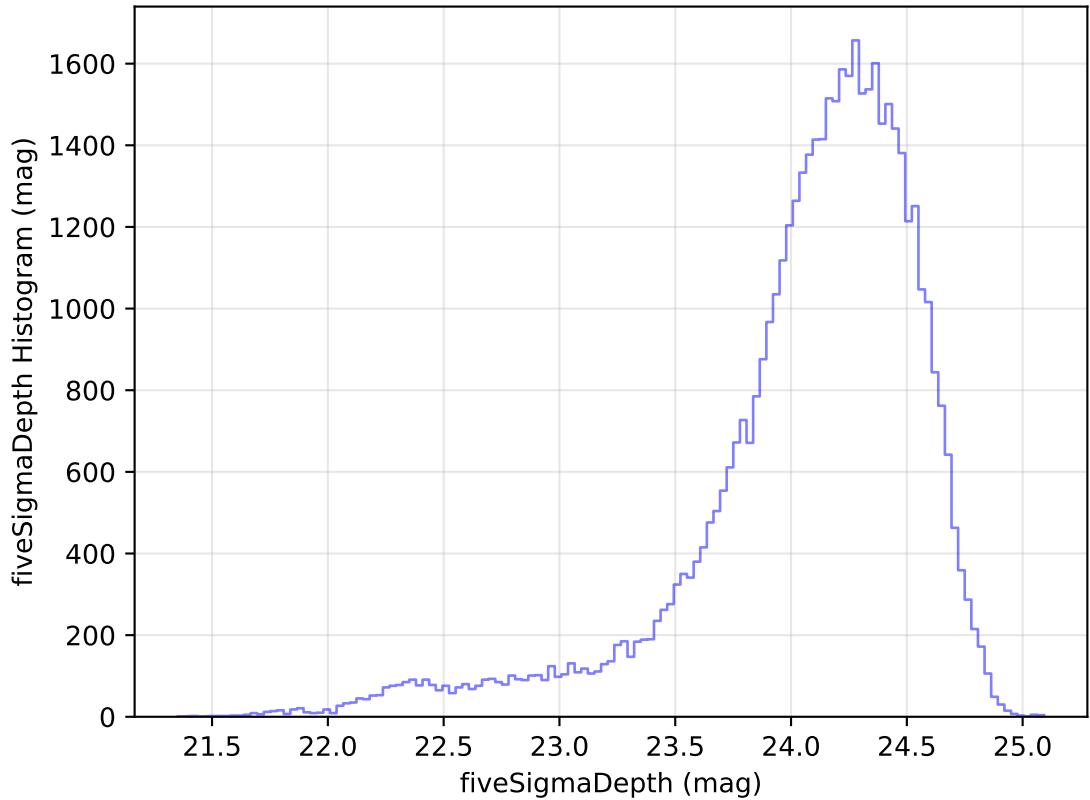
internal_u_expt27_nscale1.2v3.4_10yrs Yr 1 r band: fiveSigmaDepth Histogram
