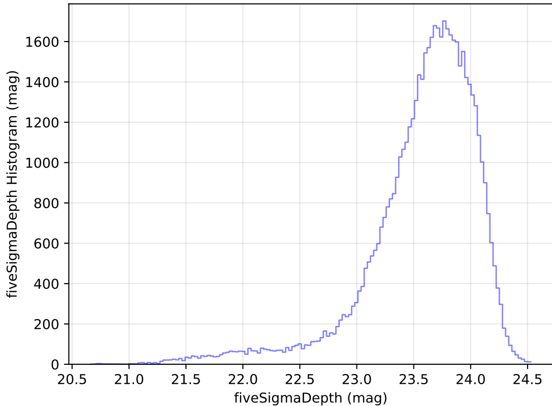
internal_u_expt27_nscale1.2v3.4_10yrs Yr 1 i band: fiveSigmaDepth Histogram
