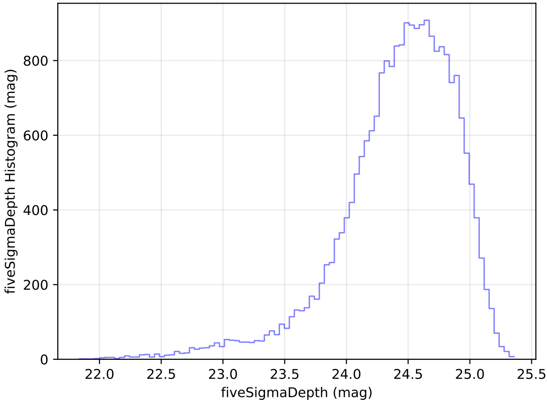
internal_u_expt27_nscale1.2v3.4_10yrs Yr 1 g band: fiveSigmaDepth Histogram
