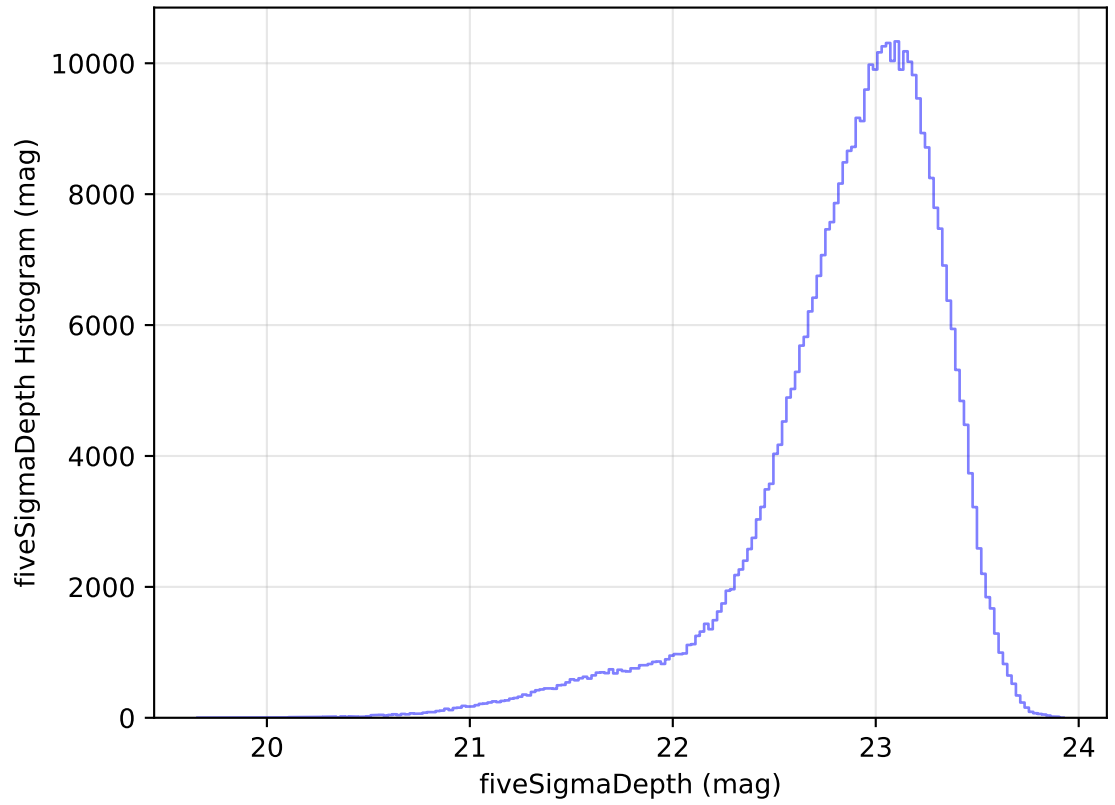
internal_u_expt27_nscale1.2v3.4_10yrs WFD z band: fiveSigmaDepth Histogram
