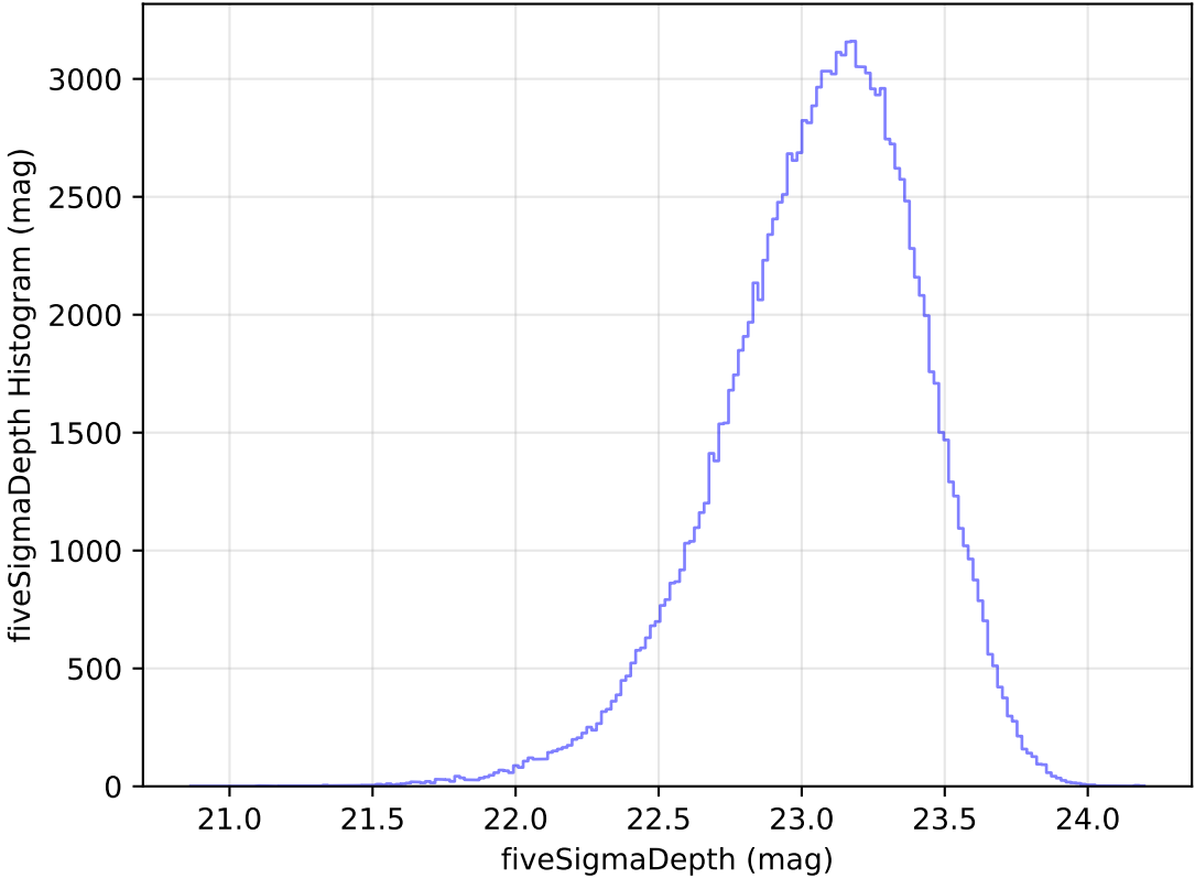
internal_u_expt27_nscale1.2v3.4_10yrs WFD u band: fiveSigmaDepth Histogram
