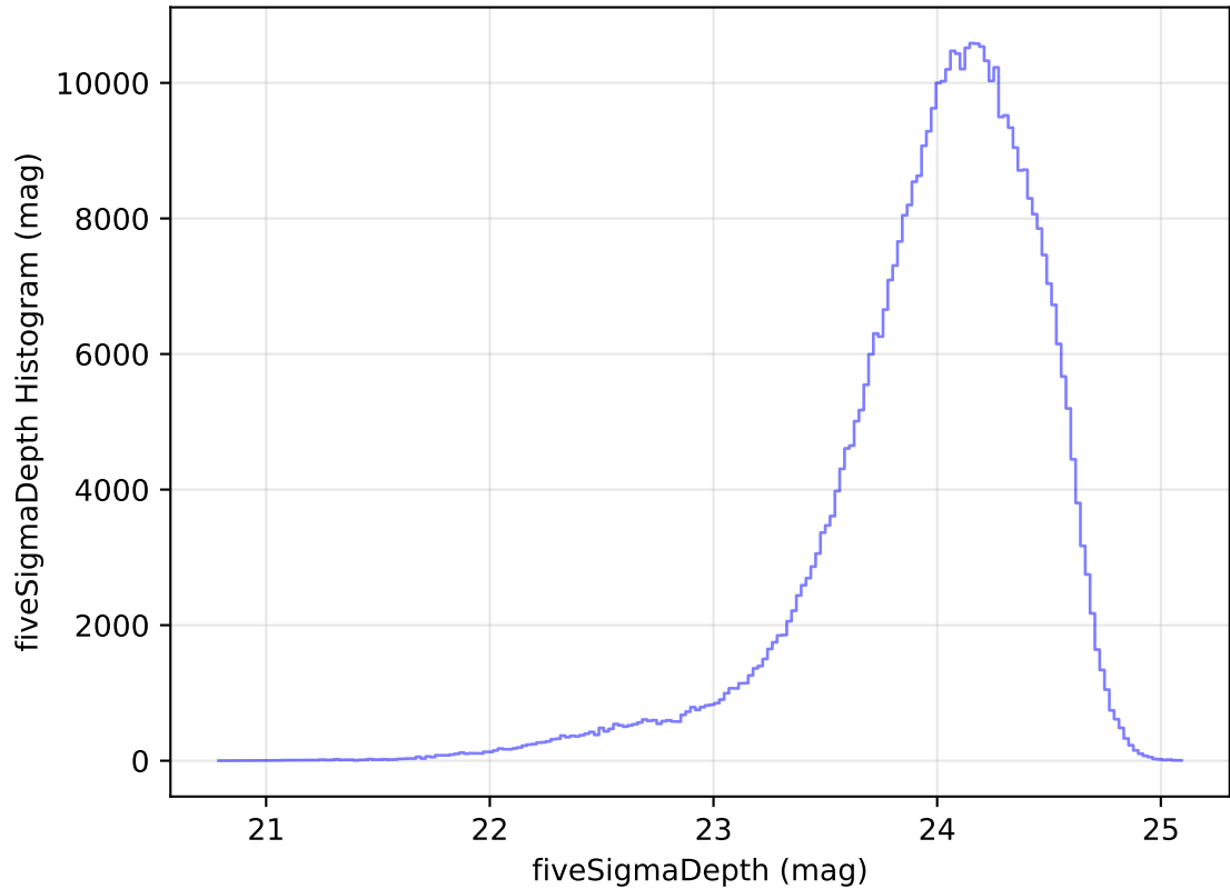
internal_u_expt27_nscale1.2v3.4_10yrs WFD r band: fiveSigmaDepth Histogram
