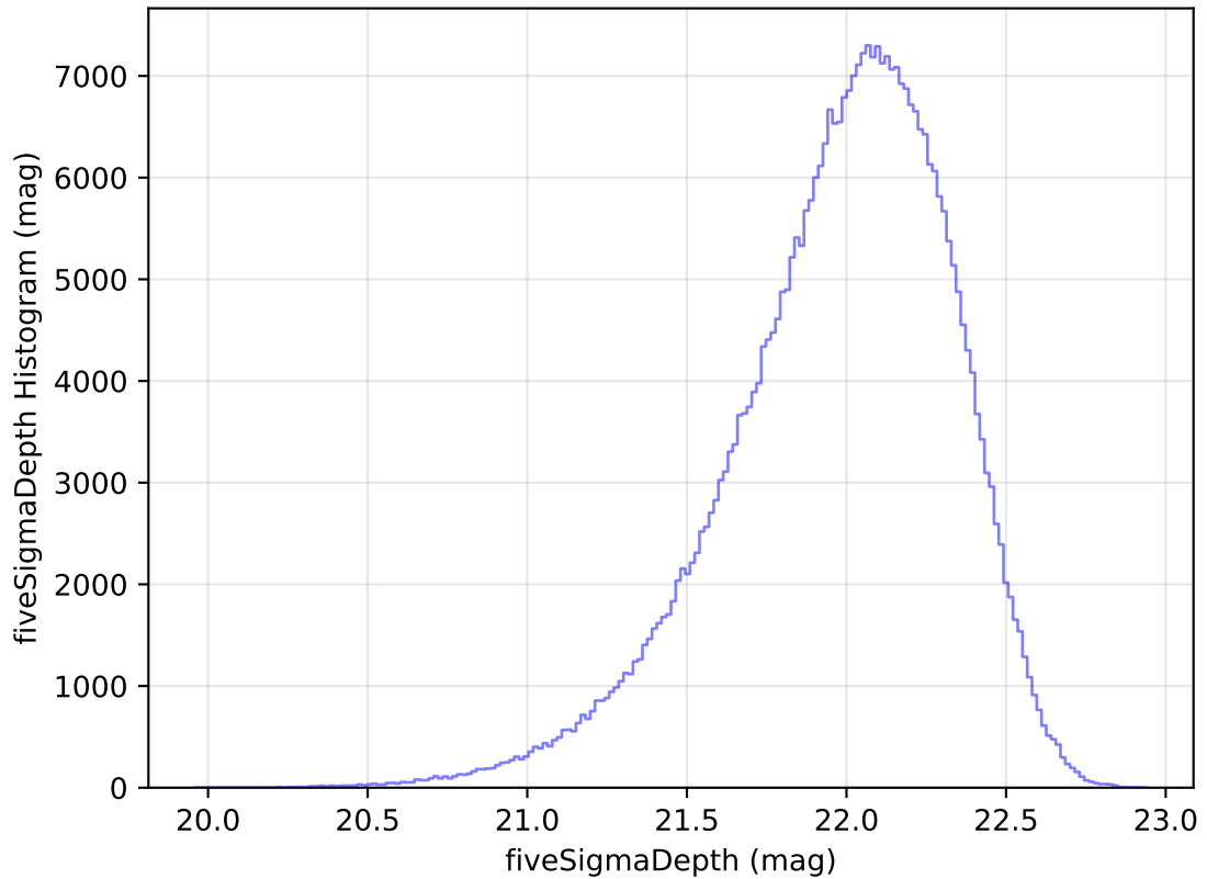
internal_u_expt27_nscale1.2v3.4_10yrs All sky y band: fiveSigmaDepth Histogram
