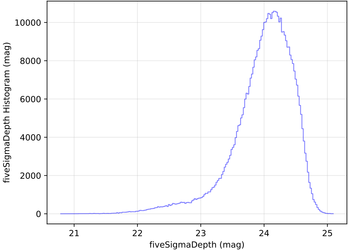
internal_u_expt27_nscale1.2v3.4_10yrs All sky r band: fiveSigmaDepth Histogram
