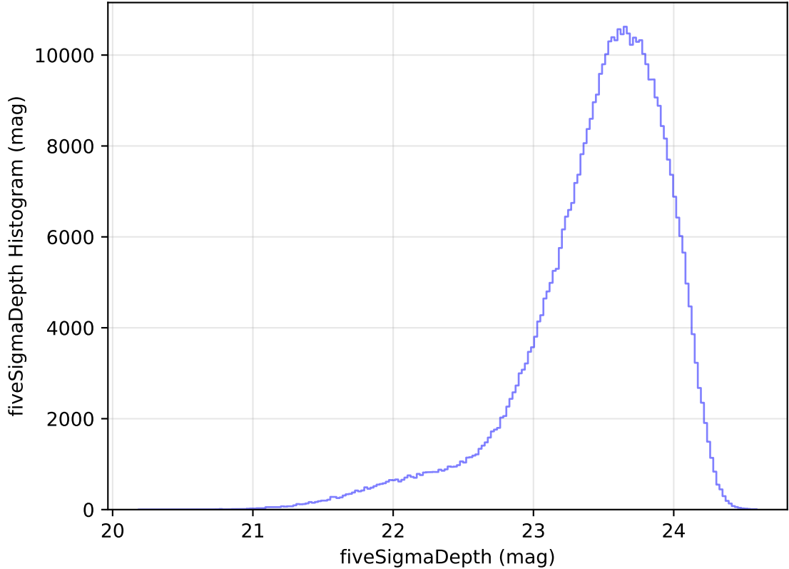
internal_u_expt27_nscale1.2v3.4_10yrs All sky i band: fiveSigmaDepth Histogram
