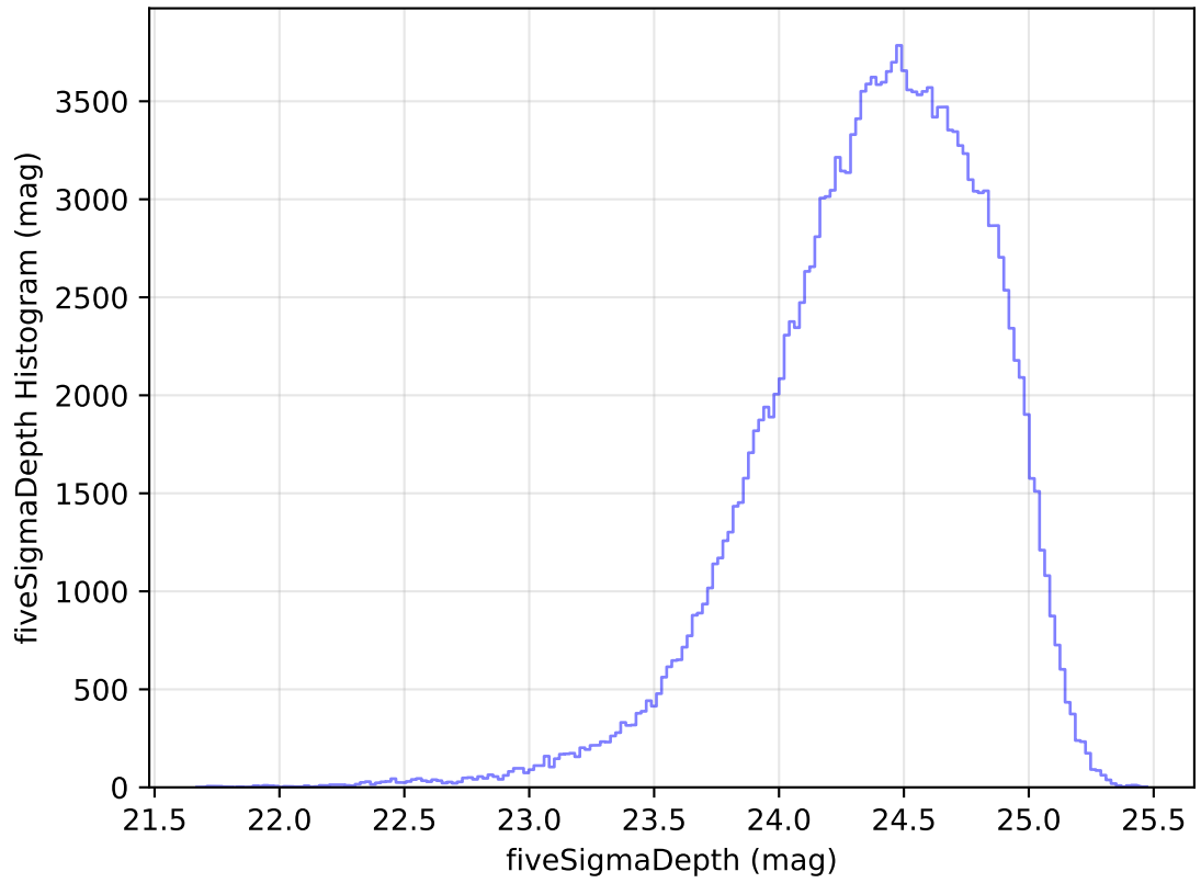
internal_u_expt27_nscale1.2v3.4_10yrs All sky g band: fiveSigmaDepth Histogram
