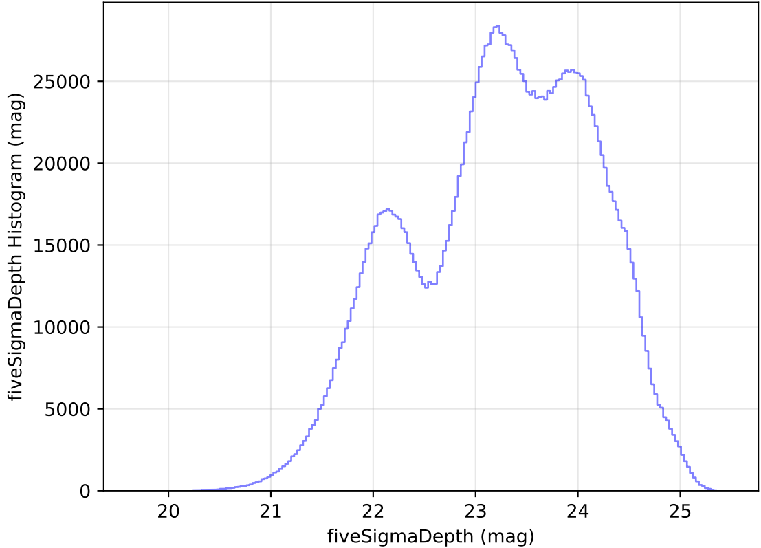
internal_u_expt27_nscale1.2v3.4_10yrs All sky all bands: fiveSigmaDepth Histogram
