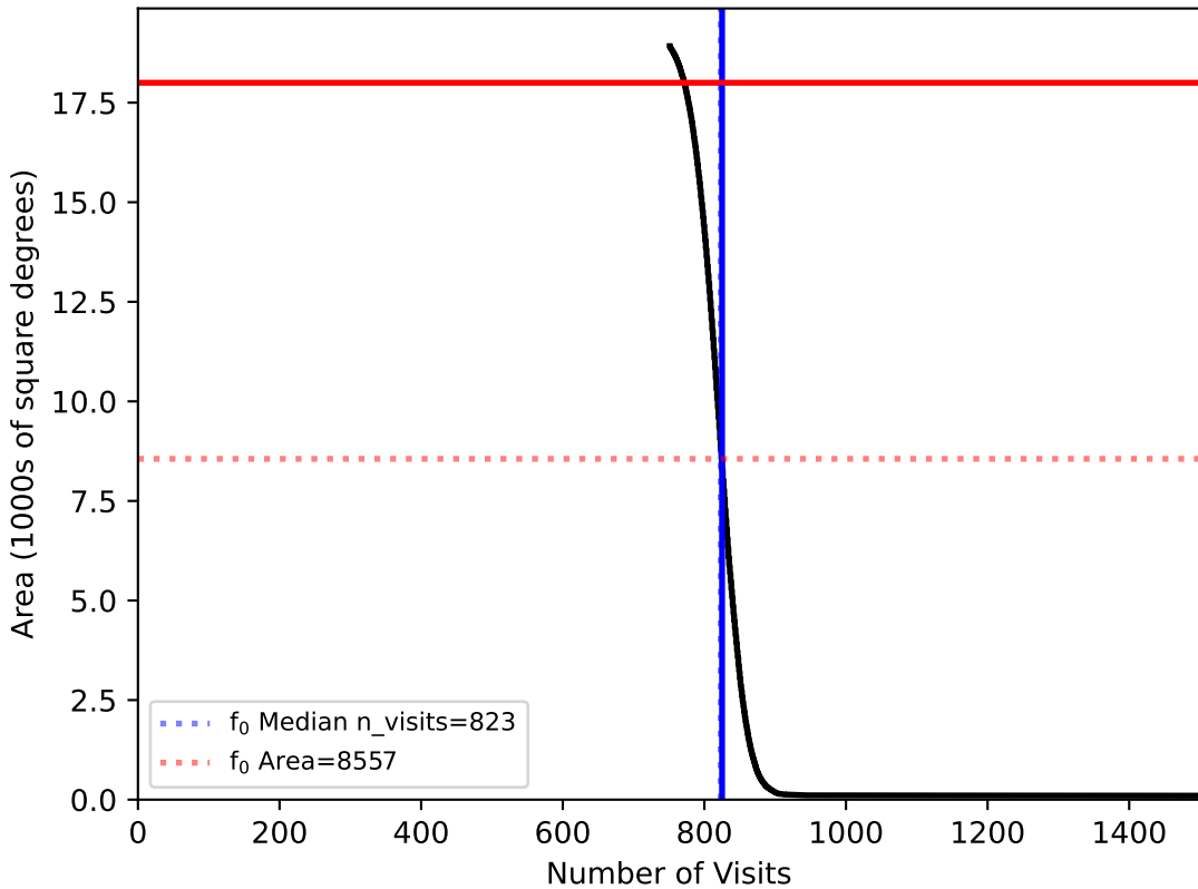
internal_u_expt27_nscale1.2v3.4_10yrs WFD: f0
