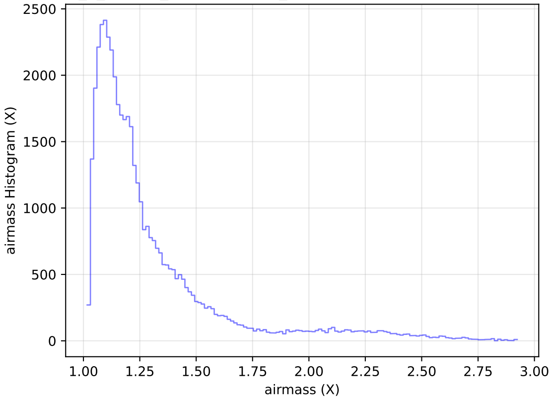
internal_u_expt27_nscale1.2v3.4_10yrs Yr 1 z band: airmass Histogram
