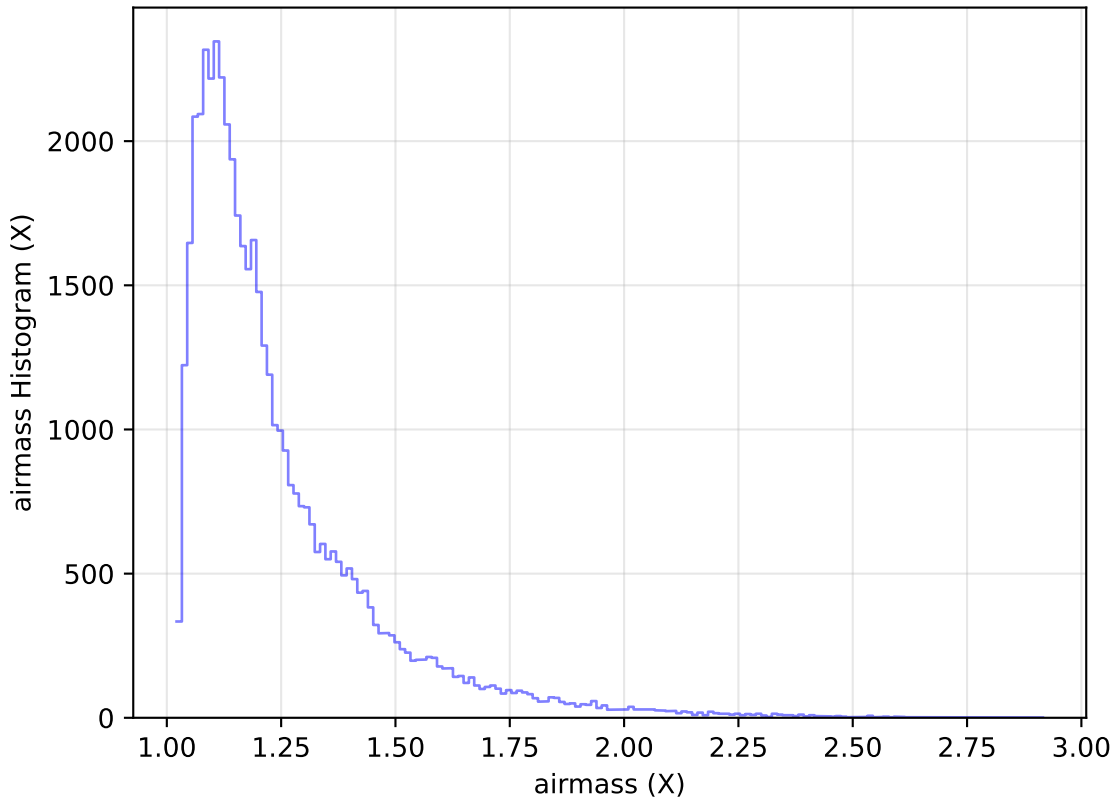
internal_u_expt27_nscale1.2v3.4_10yrs Yr 1 y band: airmass Histogram
