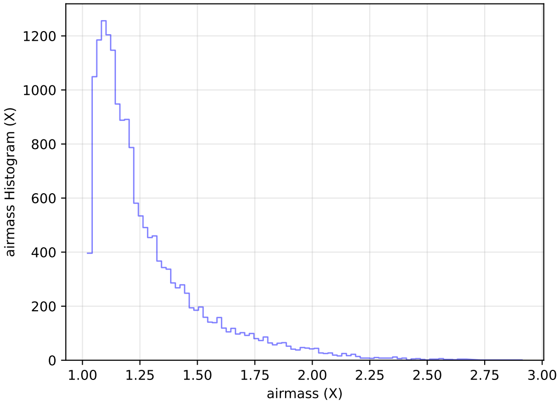
internal_u_expt27_nscale1.2v3.4_10yrs Yr 1 u band: airmass Histogram
