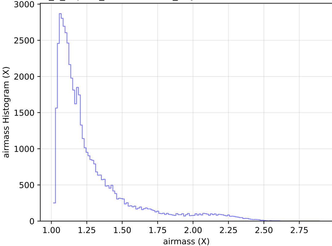
internal_u_expt27_nscale1.2v3.4_10yrs Yr 1 r band: airmass Histogram
