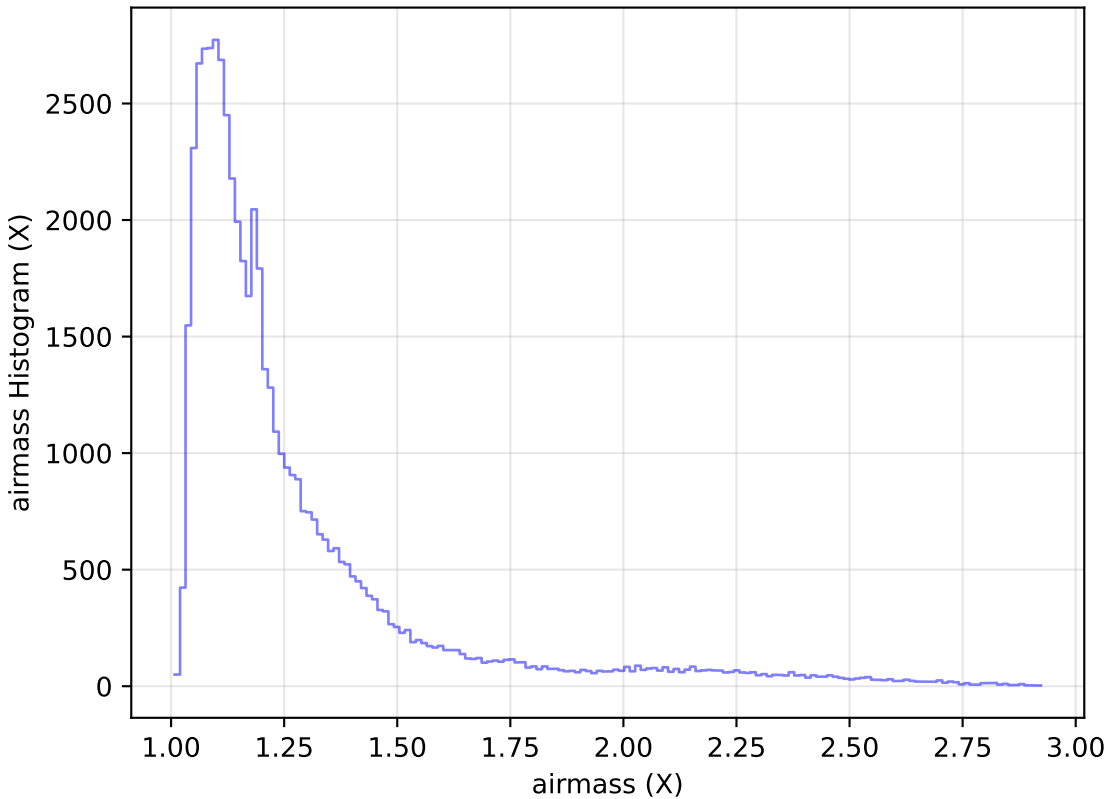
internal_u_expt27_nscale1.2v3.4_10yrs Yr 1 i band: airmass Histogram
