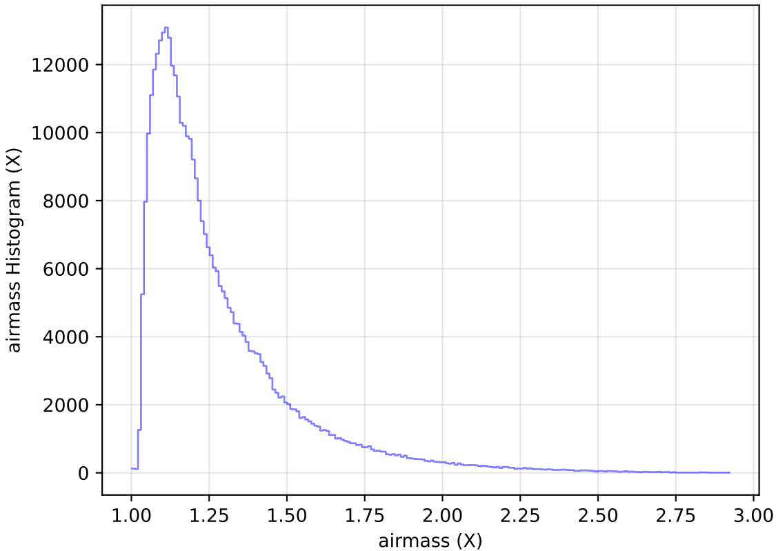
internal_u_expt27_nscale1.2v3.4_10yrs WFD y band: airmass Histogram
