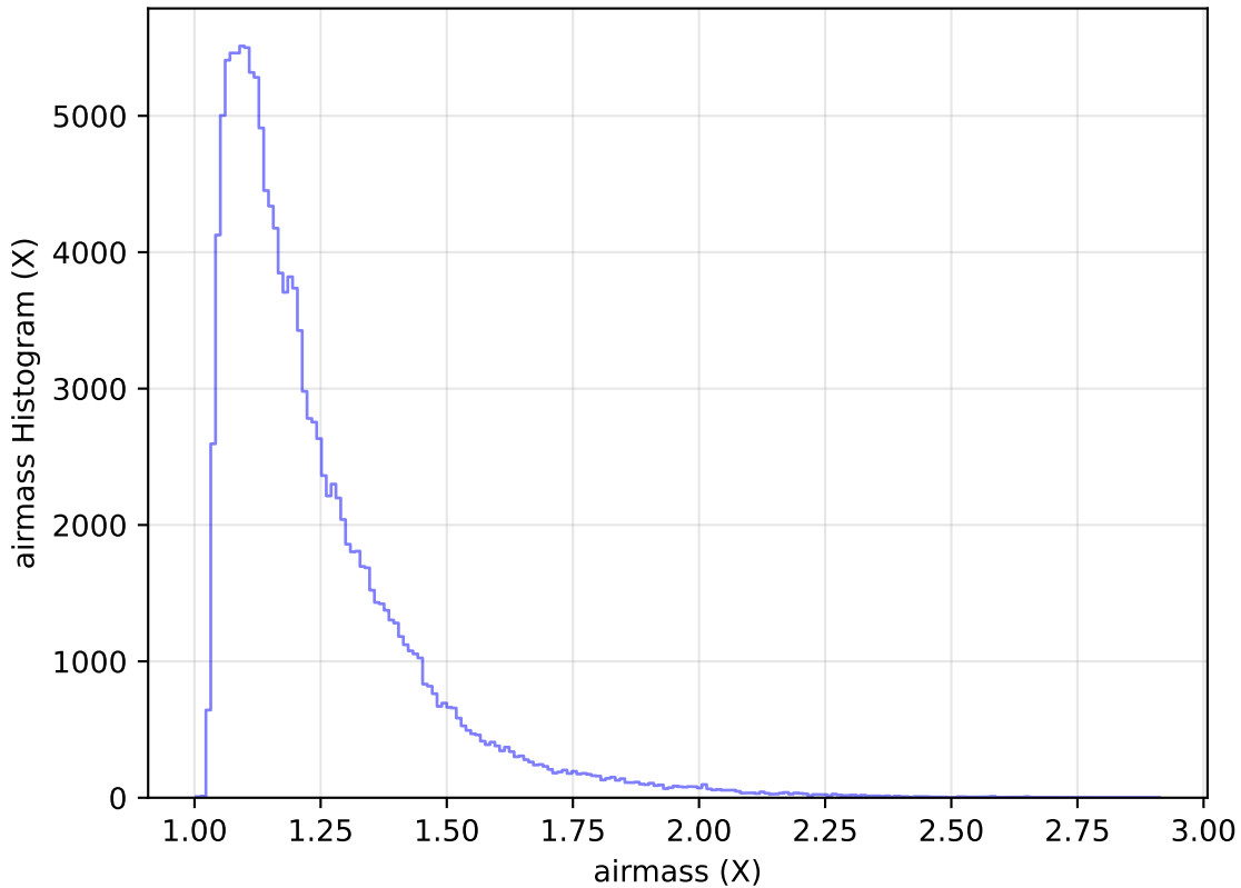
internal_u_expt27_nscale1.2v3.4_10yrs WFD u band: airmass Histogram
