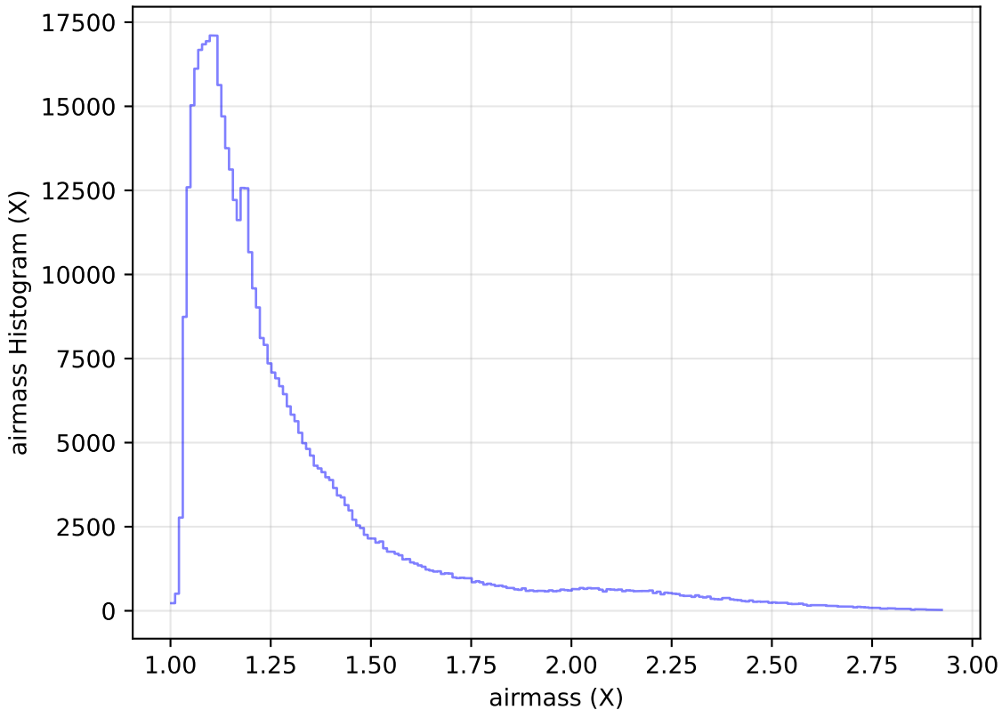
internal_u_expt27_nscale1.2v3.4_10yrs WFD i band: airmass Histogram
