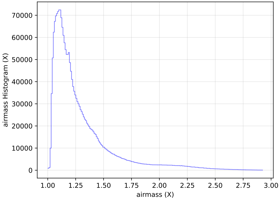
internal_u_expt27_nscale1.2v3.4_10yrs WFD all bands: airmass Histogram
