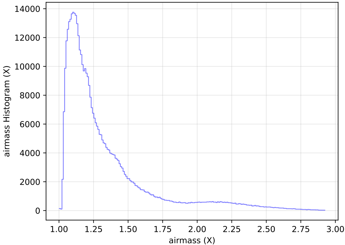
internal_u_expt27_nscale1.2v3.4_10yrs All sky z band: airmass Histogram
