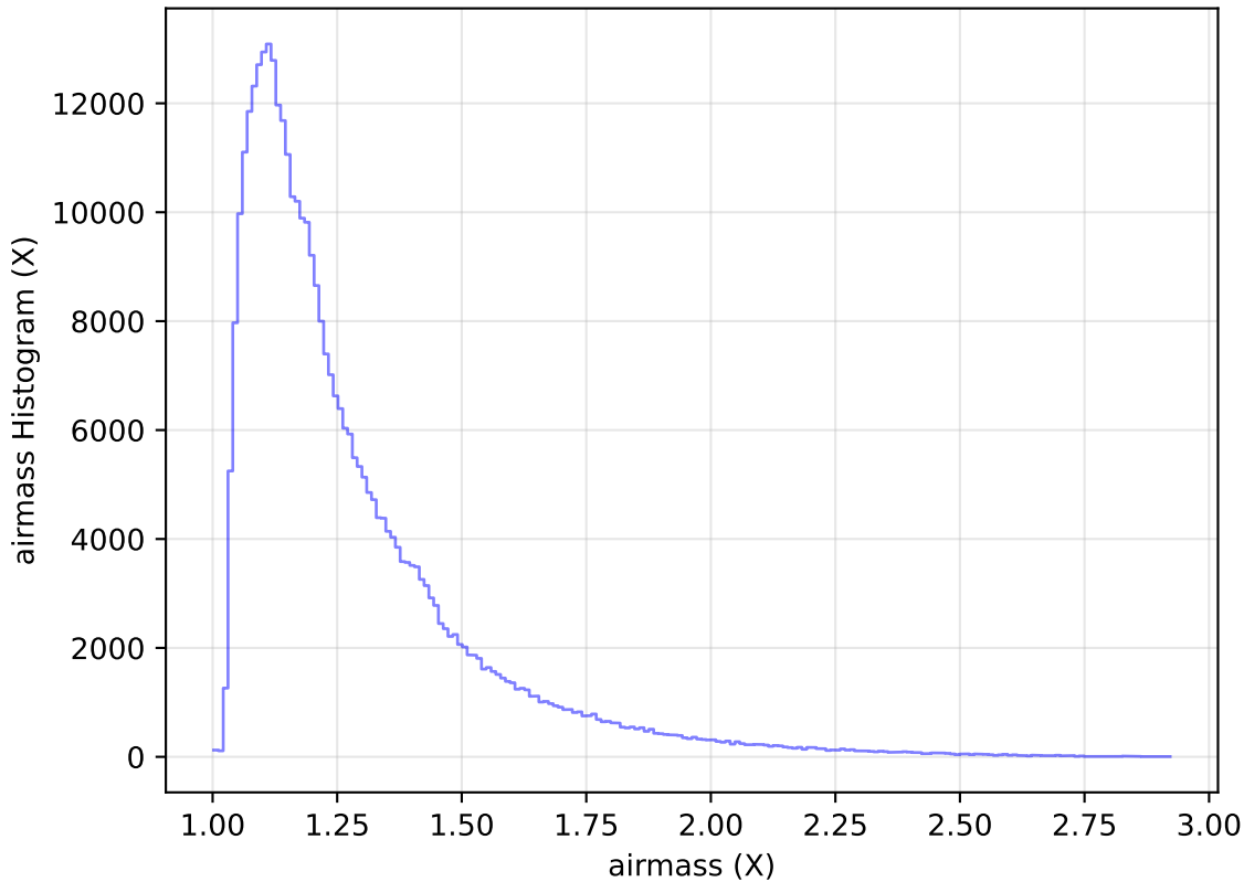
internal_u_expt27_nscale1.2v3.4_10yrs All sky y band: airmass Histogram
