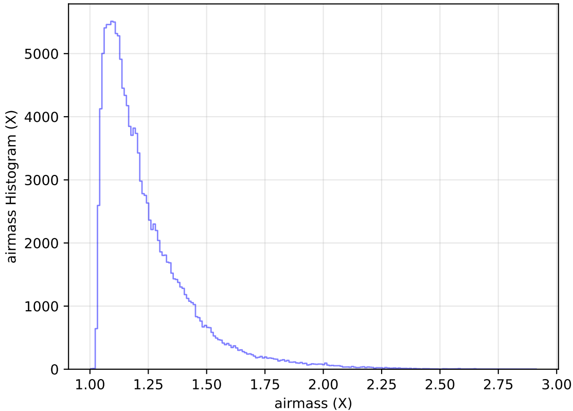
internal_u_expt27_nscale1.2v3.4_10yrs All sky u band: airmass Histogram
