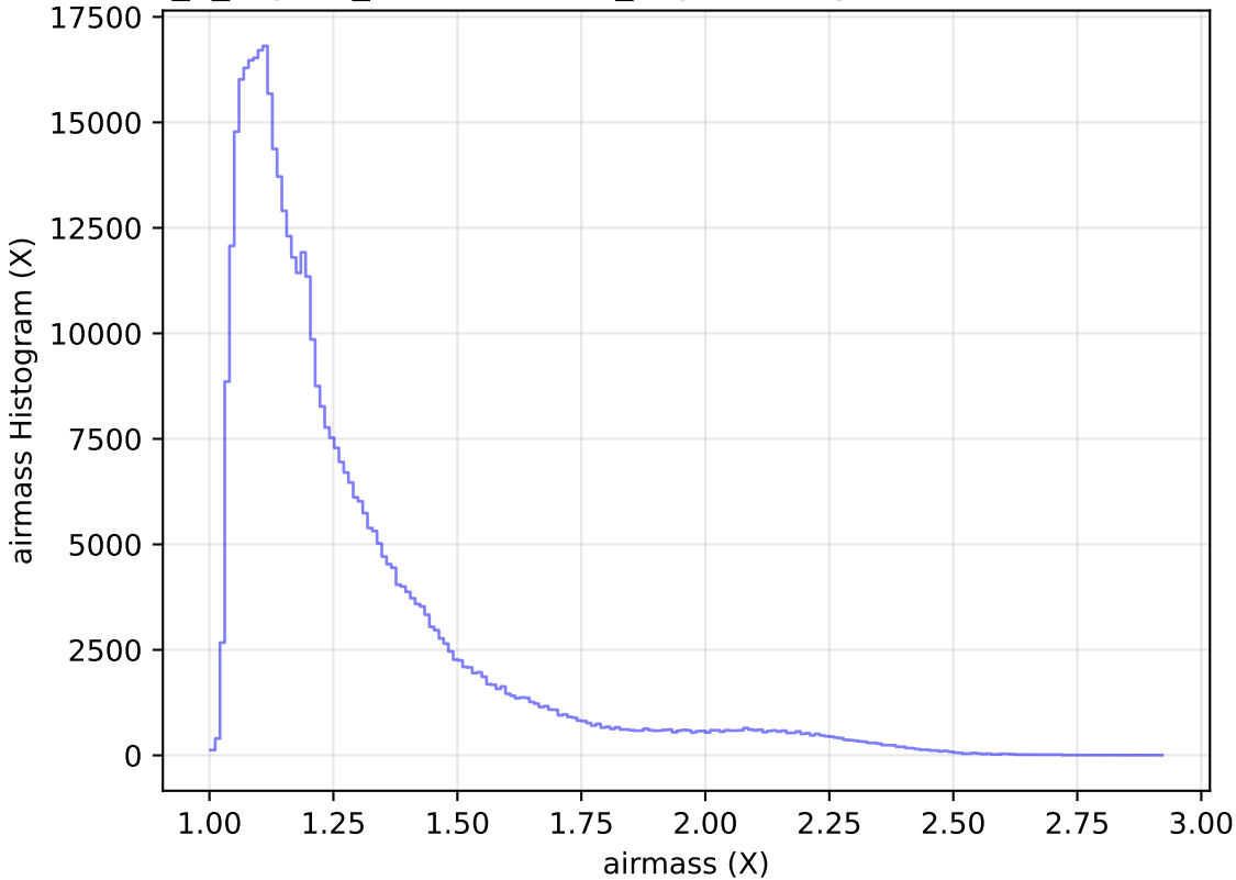
internal_u_expt27_nscale1.2v3.4_10yrs All sky r band: airmass Histogram
