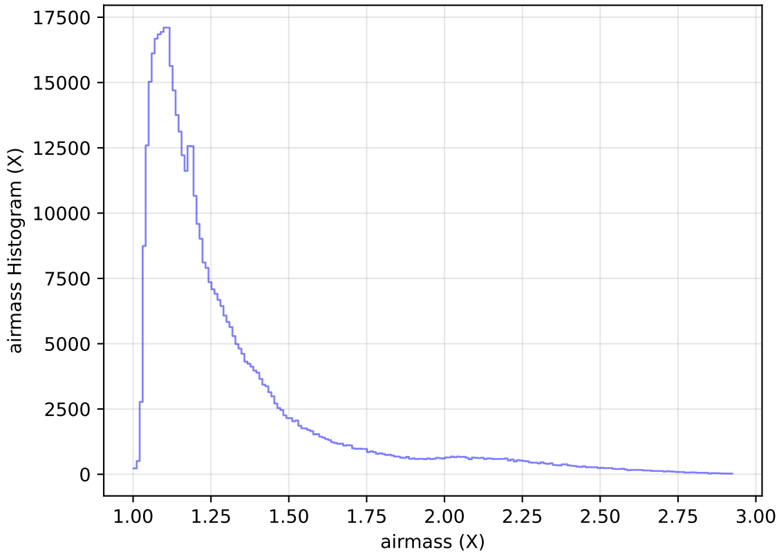
internal_u_expt27_nscale1.2v3.4_10yrs All sky i band: airmass Histogram
