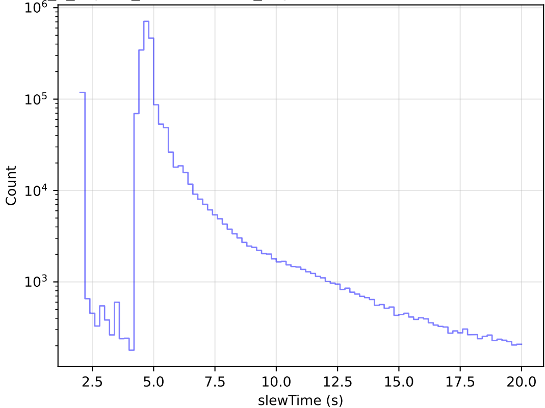
internal_u_expt27_nscale1.2v3.4_10yrs All visits: Zoom Slew Time Histogram
