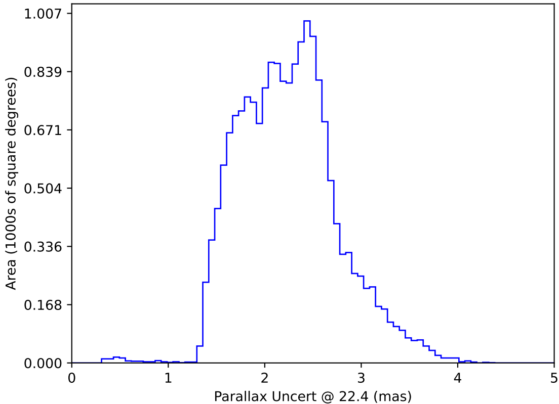
internal_u_expt27_nscale1.2v3.4_10yrs WFD: Parallax Uncert @ 22.4
