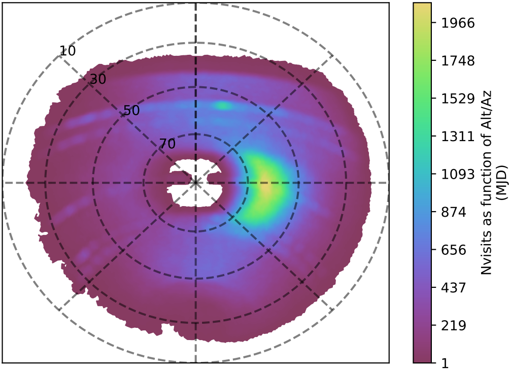
internal_u_expt27_nscale1.2v3.4_10yrs y band: Nvisits as function of Alt/Az
