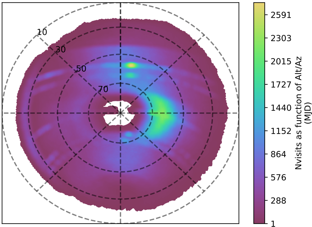
internal_u_expt27_nscale1.2v3.4_10yrs r band: Nvisits as function of Alt/Az
