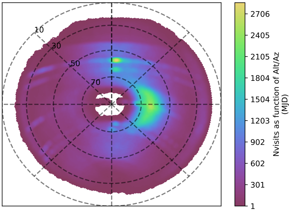
internal_u_expt27_nscale1.2v3.4_10yrs i band: Nvisits as function of Alt/Az
