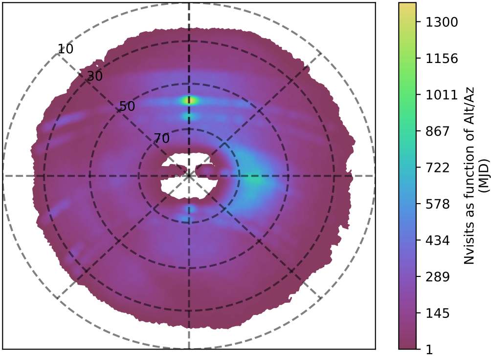
internal_u_expt27_nscale1.2v3.4_10yrs g band: Nvisits as function of Alt/Az
