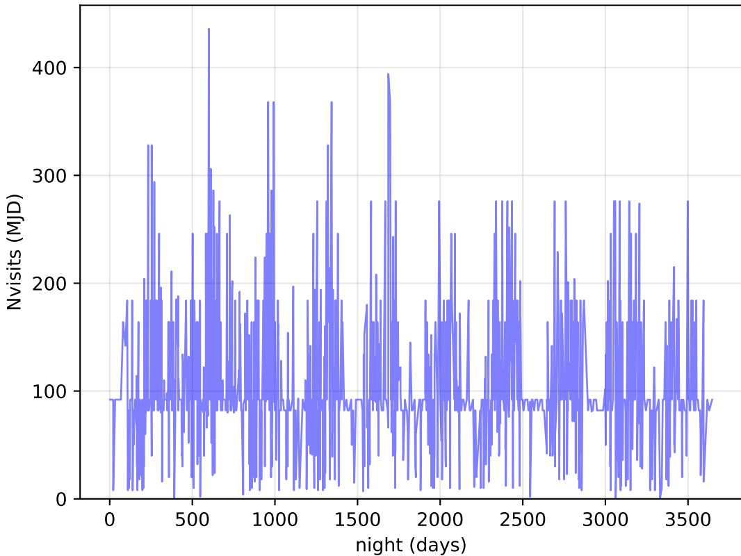
internal_u_expt27_nscale1.2v3.4_10yrs DDF: Nvisits
