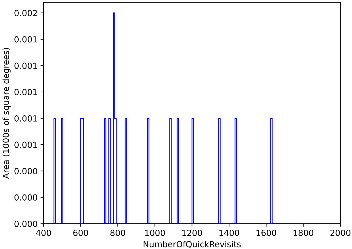
internal_u_expt27_nscale1.2v3.4_10yrs WFD: NumberOfQuickRevisits
