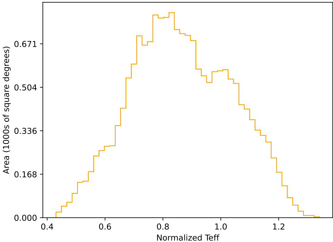
internal_u_expt27_nscale1.2v3.4_10yrs WFD r band: Normalized Teff
