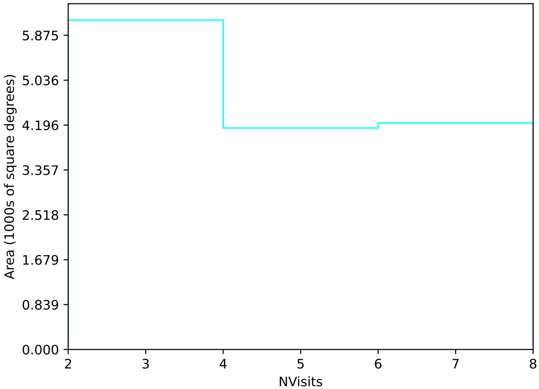
internal_u_expt27_nscale1.2v3.4_10yrs Yr 3-4 u band: NVisits
