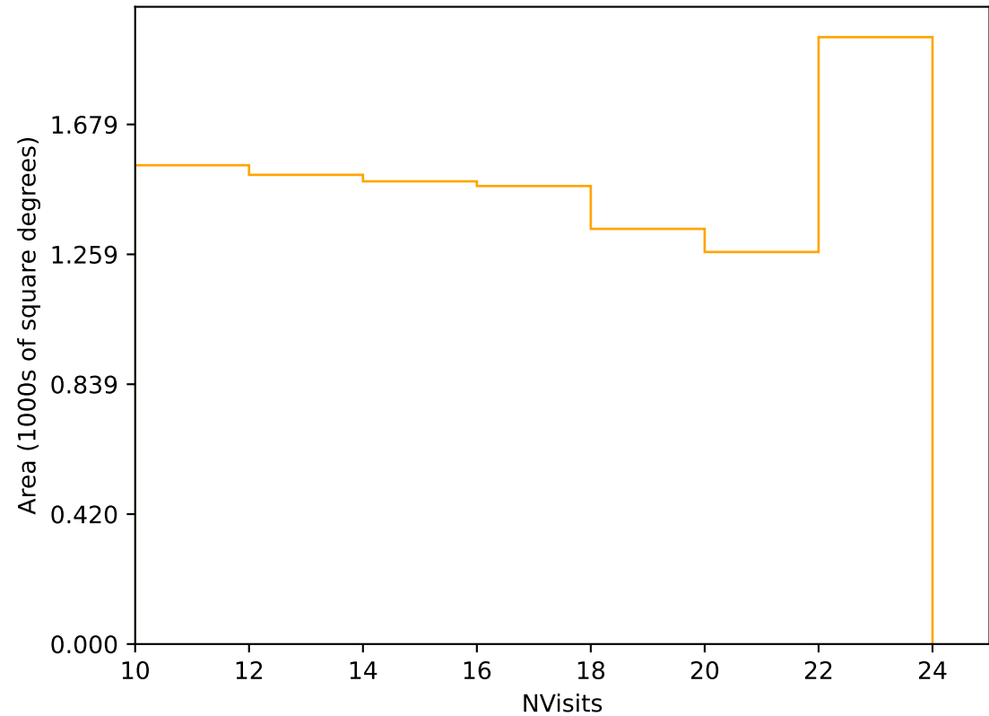
internal_u_expt27_nscale1.2v3.4_10yrs Yr 3-4 r band: NVisits
