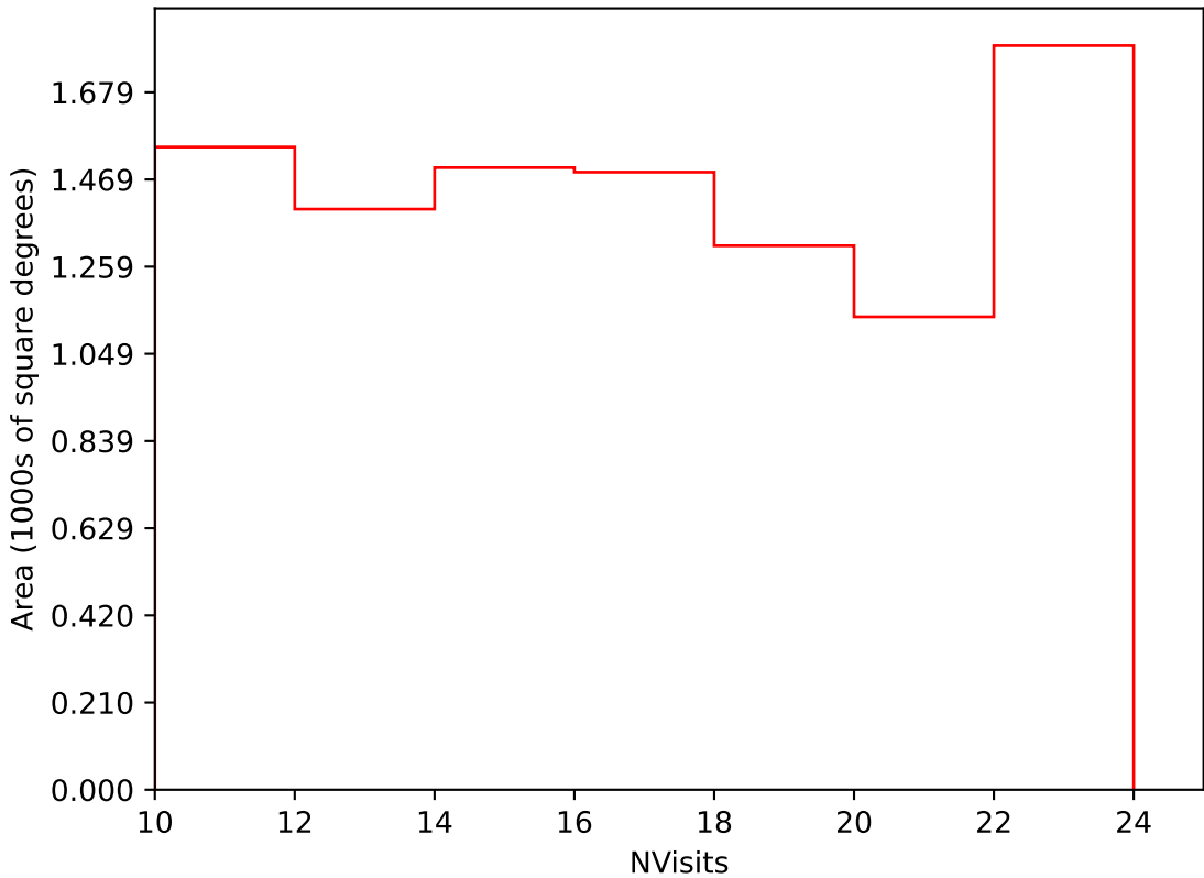
internal_u_expt27_nscale1.2v3.4_10yrs Yr 3-4 i band: NVisits
