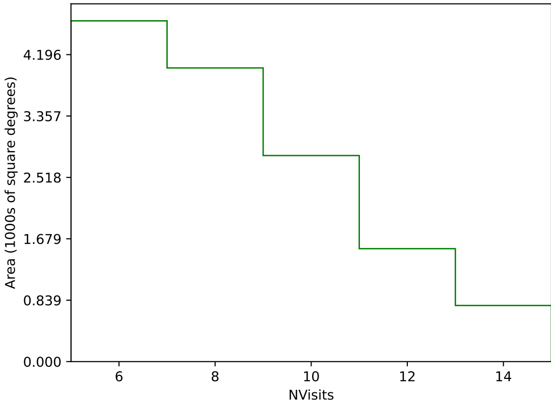
internal_u_expt27_nscale1.2v3.4_10yrs Yr 3-4 g band: NVisits
