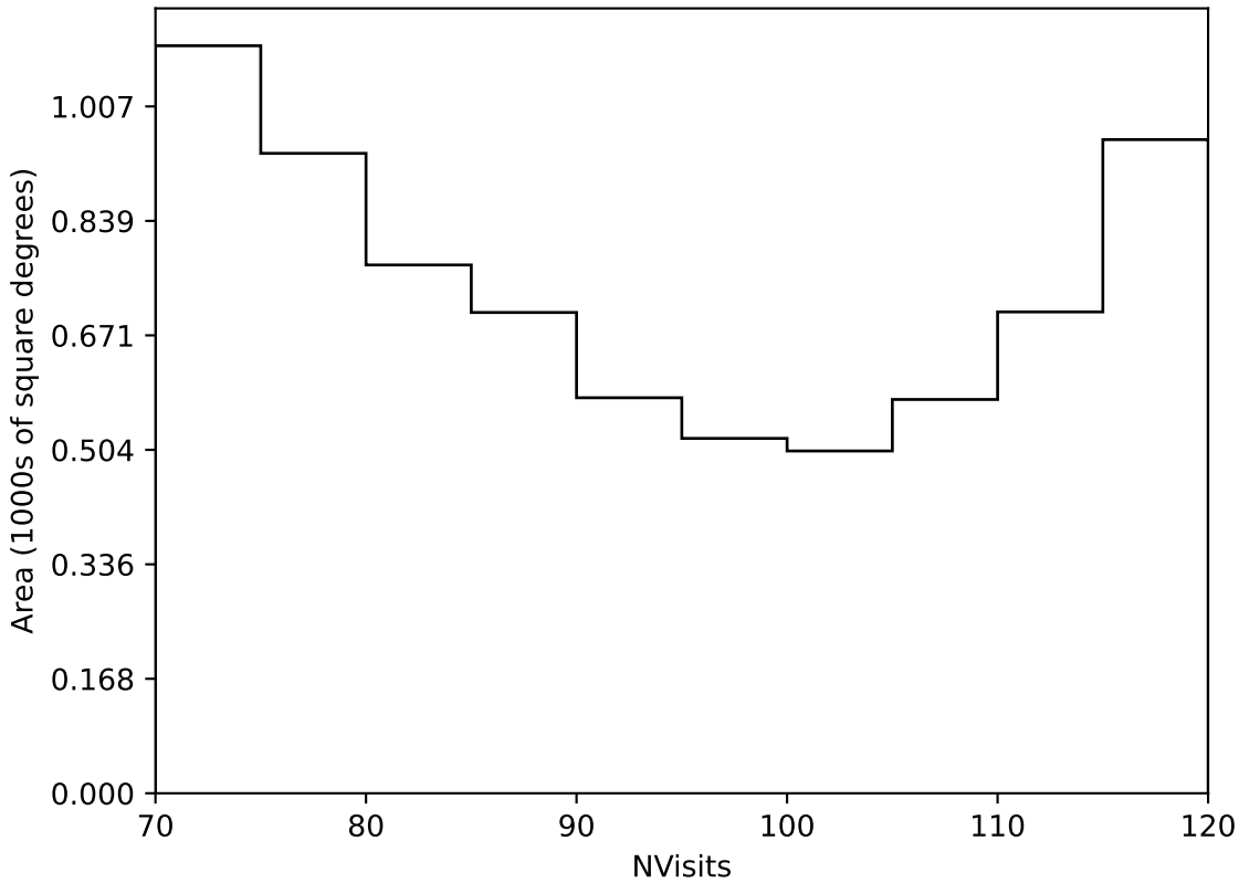
internal_u_expt27_nscale1.2v3.4_10yrs Yr 3-4 all bands: NVisits
