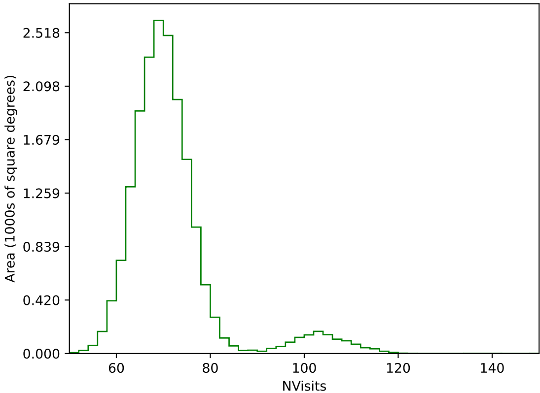
internal_u_expt27_nscale1.2v3.4_10yrs WFD g band: NVisits
