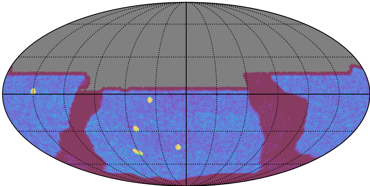
internal_u_expt27_nscale1.2v3.4_10yrs All sky y band: NVisits
