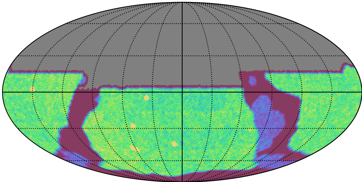
internal_u_expt27_nscale1.2v3.4_10yrs All sky u band: NVisits
