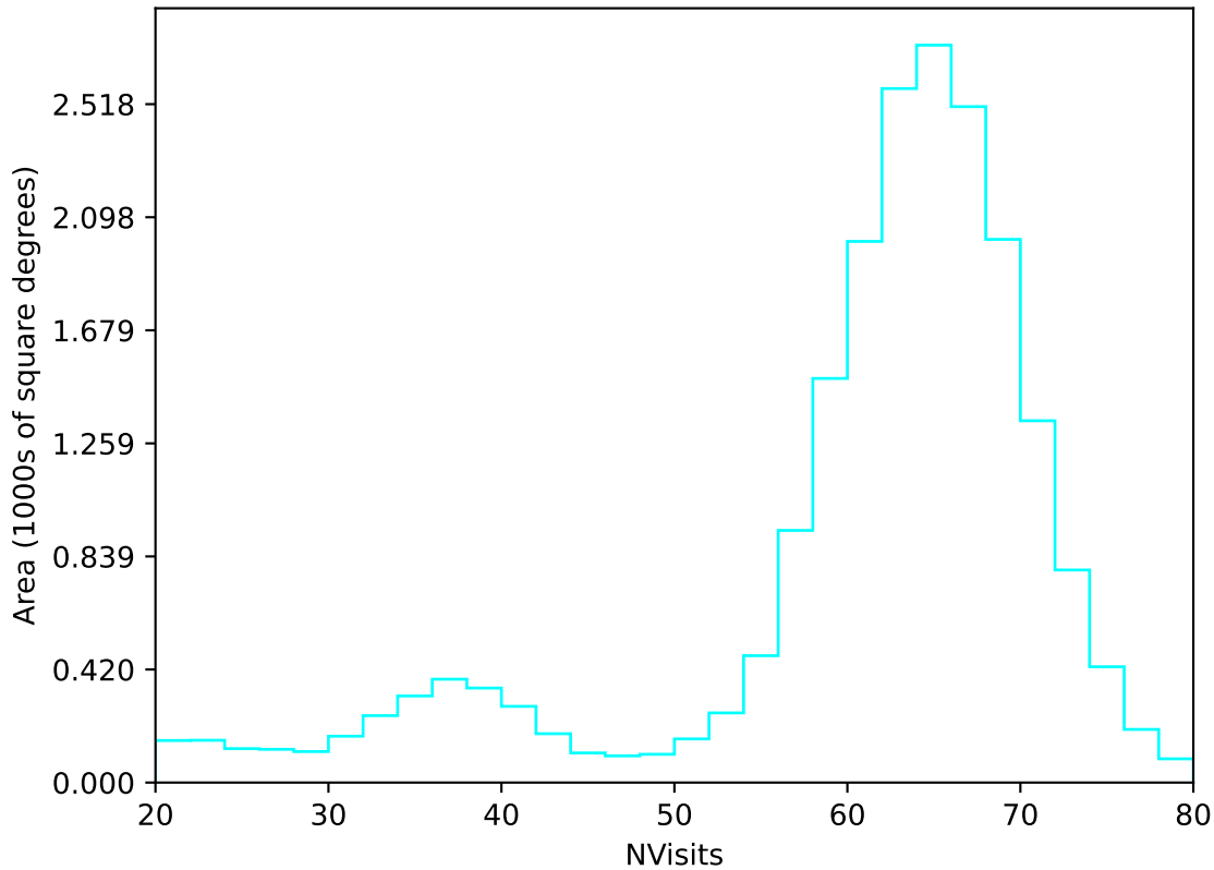
internal_u_expt27_nscale1.2v3.4_10yrs All sky u band: NVisits
