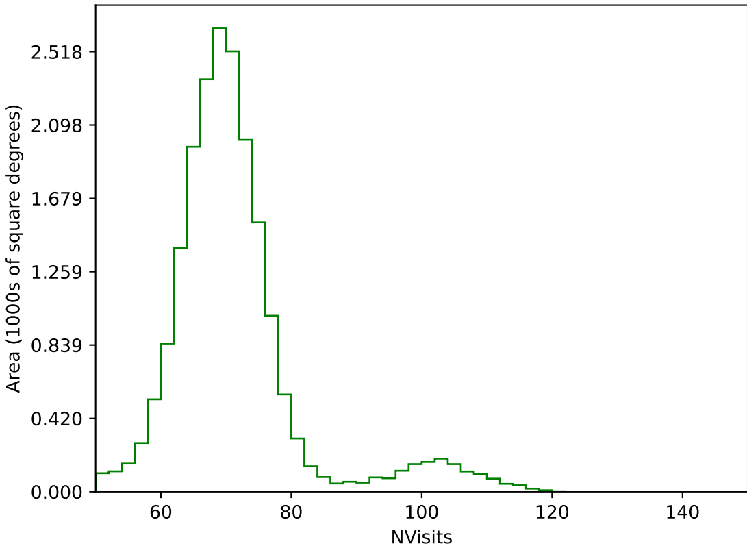
internal_u_expt27_nscale1.2v3.4_10yrs All sky g band: NVisits
