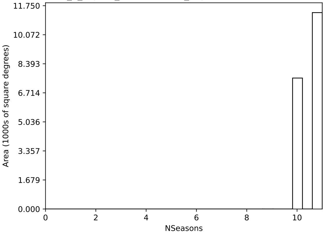
internal_u_expt27_nscale1.2v3.4_10yrs WFD all bands: NSeasons
