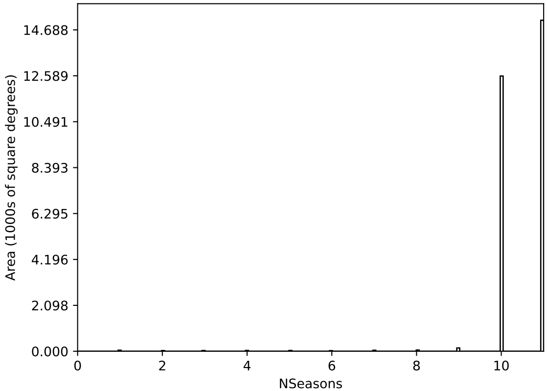
internal_u_expt27_nscale1.2v3.4_10yrs All sky all bands: NSeasons
