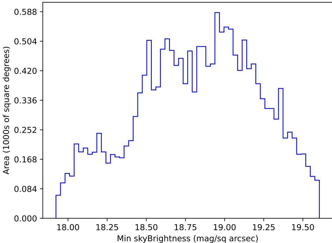
internal_u_expt27_nscale1.2v3.4_10yrs WFD r band: Min skyBrightness
