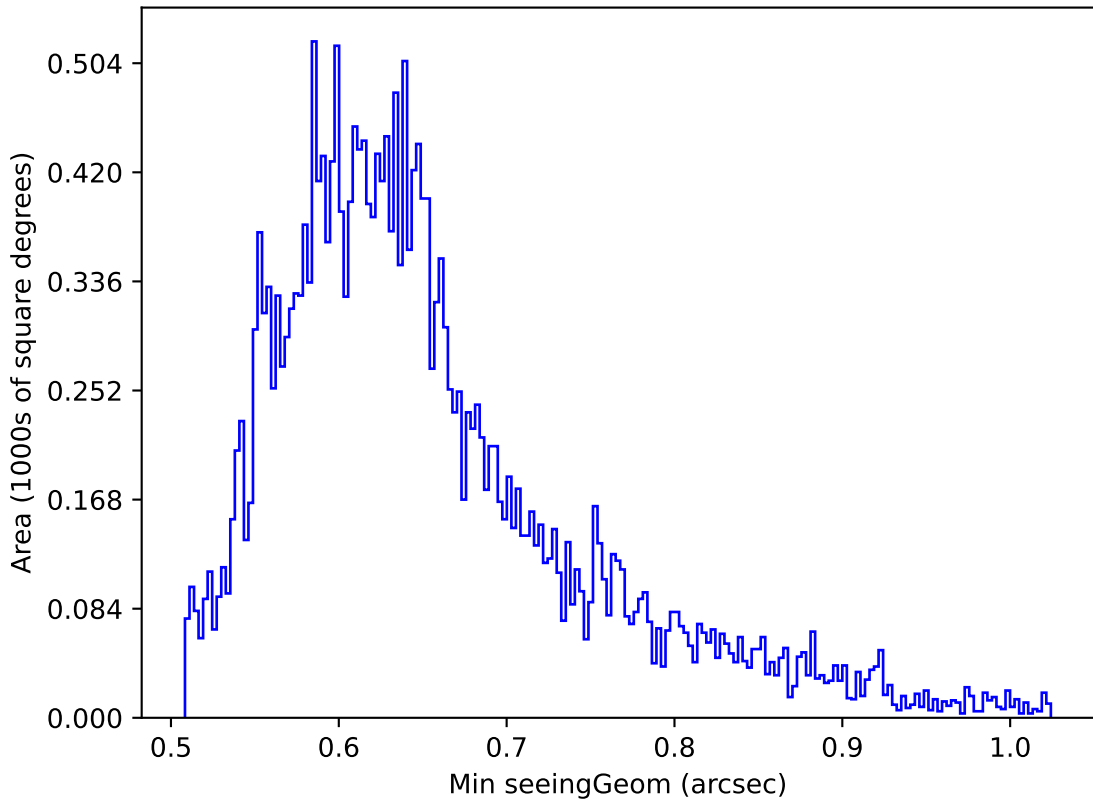
internal_u_expt27_nscale1.2v3.4_10yrs Yr 1 z band: Min seeingGeom
