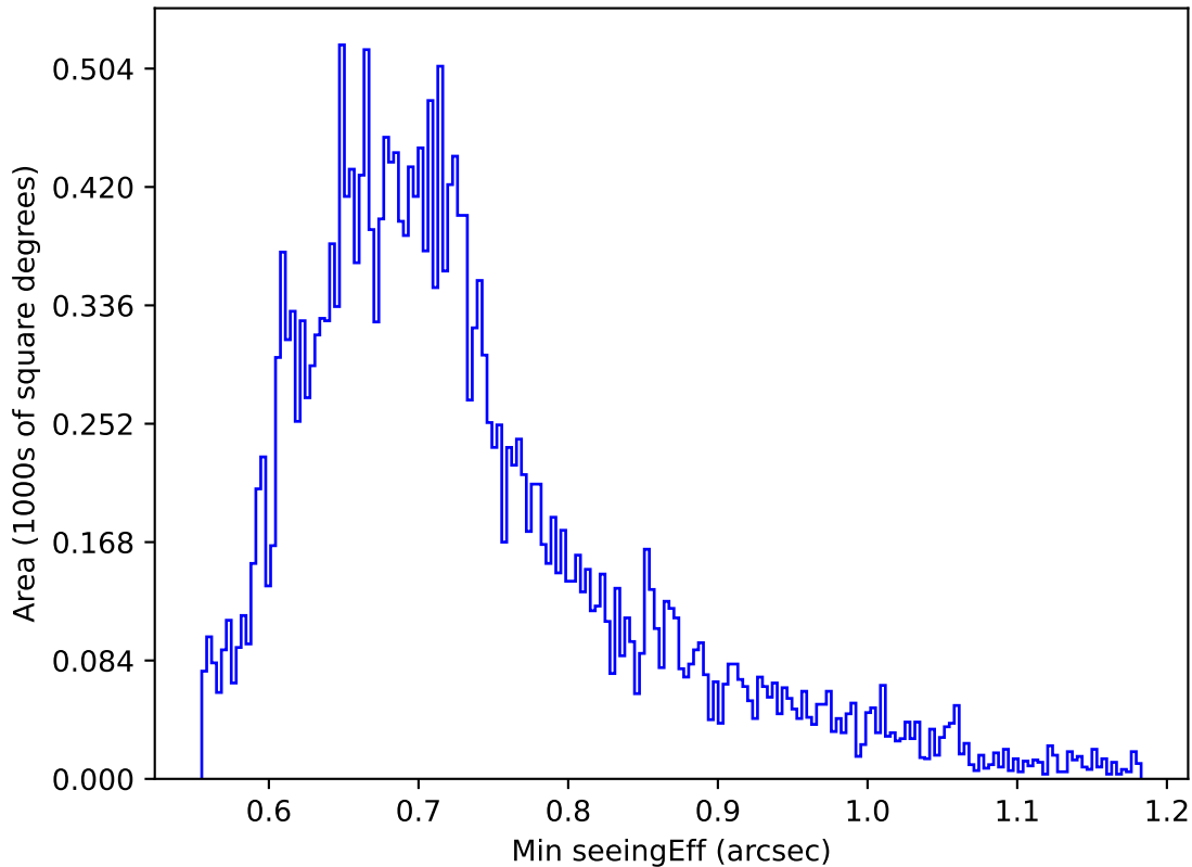
internal_u_expt27_nscale1.2v3.4_10yrs Yr 1 z band: Min seeingEff
